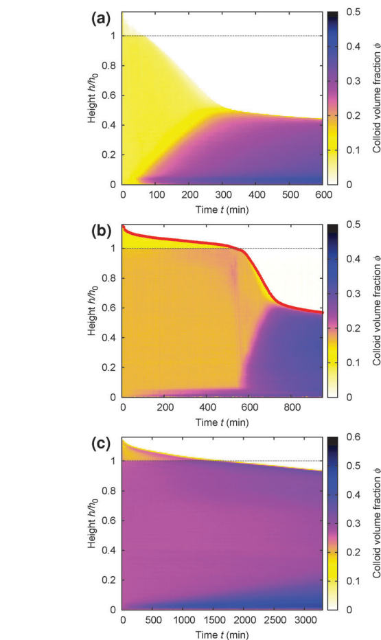
Fig. 8 Time evolution of the height profile, \phi(z) , from MRI. In all cases, the dashed horizontal line marks the bottom of the meniscus ( h_0 in Fig. 2). (a) A typical sample showing type A gravitational collapse. (b) A typical sample showing regime D gravitational collapse. The time-dependent height profile of this sample, picked out in red, is reproduced in Fig. 9(a). (c) A sample just inside regime B.
