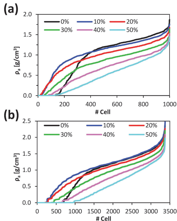
Fig. 4 Local apparent density ( \rho_a ) for the (a) 1000 and (b) 3375 cells in which microstructures were divided. Cells were ranked following a growing local density order.
