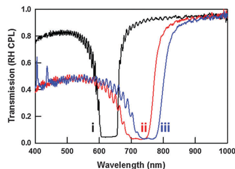
Fig. 7 Photosensitivity of t-PSCLC prepared with the photoinitiator I-907 (1 wt%). Transmission spectra at (i) 0 V (—), (ii) during application of 40 V DC (—), and during application of 40 V DC in the presence of 50 mW cm -2 of UV light (—).
