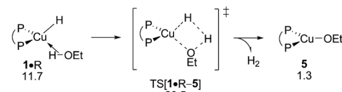
Fig. 13 Protonolysis of ethanol by the \{\text{P}^\wedge\text{P}\}\text{Cu}^{\text{I}} hydride. 19,20 Free energies are given in \text{kcal mol}^{-1} relative to \{\frac{1}{2}\mathbf{1dim} + \text{reactants}\} .
