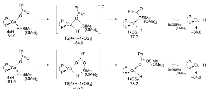
Fig. 6 Transmetalation of the \{P^AP\}Cu^I benzoate 4 with hydrosilane H. 19,20 Free energies are given in \text{kcal mol}^{-1} relative to \{1_{\text{dim}} + \text{reactants}\} .
