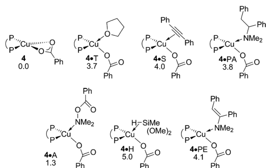
Fig. 5 Various forms of the \{P^AP\}Cu^I benzoate compound 4 . 19 Free energies are given in \text{kcal mol}^{-1} relative to \{4 + \text{reactants}\} .
