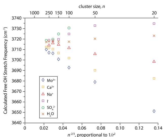
Fig. 6 Centroid frequencies of the AAD free OH bands from simulated spectra of (\text{H}_2\text{O})_n and M(\text{H}_2\text{O})_n where M = \text{Mo}^{3+} , \text{Ca}^{2+} , \text{Na}^+ , \text{I}^- and \text{SO}_4^{2-} as a function of n^{-2/3} , which is proportional to 1/r^2 where r is the droplet radius.
