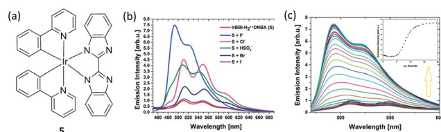
Fig. 5 (a) Chemical structure of complex 5 . (b) Luminescence intensity of \text{IrBBI-H}_2^+ \cdots \text{DNBA}^- with 110 equiv. of different anions. (c) Luminescence of \text{IrBBI-H}_2^+ \cdots \text{DNBA}^- as a function of different concentration of fluoride; inset: plot of the normalized \text{IrBBI-H}_2^+ \cdots \text{DNBA}^- luminescence response as a function of the number of equivalents of fluoride added. 54 Reprinted figures with permission from Copyright (2015) Royal Society of Chemistry.
