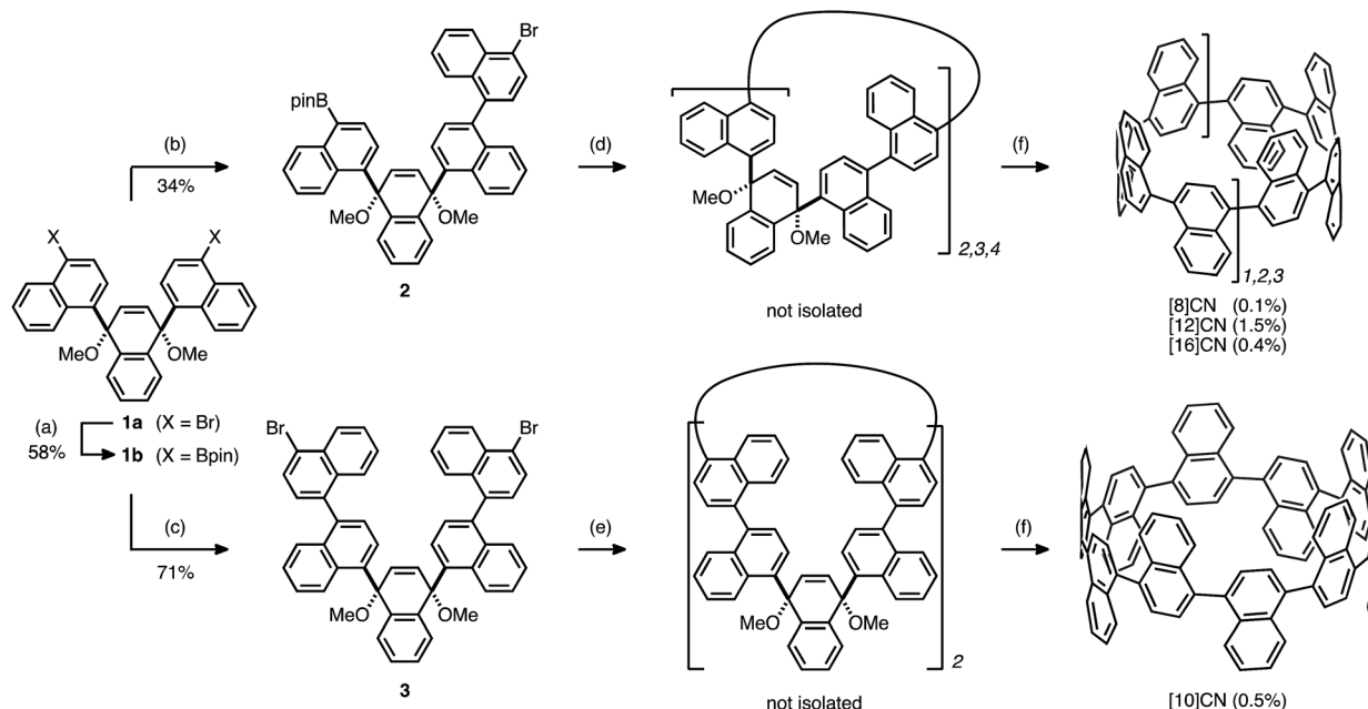
Scheme 1 Synthesis of [8]-, [10]-, [12]-, and [16]CNs. Reaction conditions: (a) 1a (1 equiv.), B 2 pin 2 (2.5 equiv.), PdCl 2 (dppf)·CH 2 Cl 2 (5 mol%), KOAc (6 equiv.), 1,4-dioxane, 90 °C, 10 h. (b) 1b (1 equiv.), 1,4-dibromonaphthalene (2.5 equiv.), Pd(PPh 3 ) 4 (10 mol%), K 2 CO 3 (5 equiv.), toluene/EtOH/H 2 O, 90 °C, 5 h. (c) 1b (1 equiv.), 1,4-dibromonaphthalene (5 equiv.), Pd(PPh 3 ) 4 (10 mol%), K 2 CO 3 (5 equiv.), toluene/EtOH/H 2 O, 90 °C, 16 h. (d) 2 (1 equiv.), Pd(PPh 3 ) 4 (10 mol%), K 2 CO 3 (5 equiv.), toluene/EtOH/H 2 O, 90 °C, 26 h. (e) 3 (1 equiv.), Ni(cod) 2 (2.2 equiv.), 2,2'-bipyridyl (2.2 equiv.), DMF, 90 °C, 24 h. (f) Li (excess), THF, rt, 12 h. Bpin = 4,4,5,5-tetramethyl-1,3,2-dioxaborolan-2-yl.
