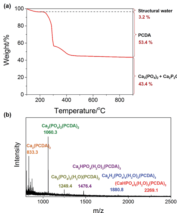
Fig. 4 (a) TGA curve (under air flow) and (b) MALDI-TOF MS of PCDA monolayer protected \text{Ca}_x(\text{PO}_4)_y cluster. For identification, corresponding assignments for the main peaks in MALDI-TOF MS are labelled.
