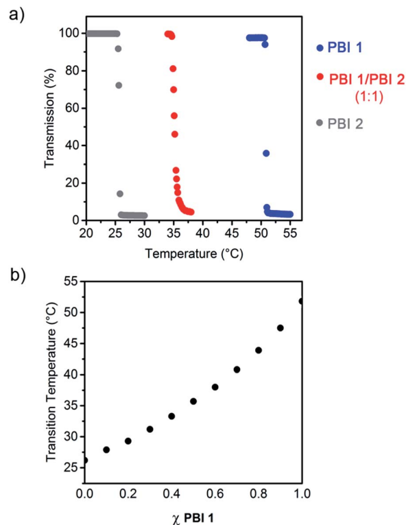
Fig. 2 (a) Transmission at 800 nm of aqueous solutions ( 2.5 \times 10^{-4} M) of PBI 1 , PBI 2 and PBI 1/PBI 2 (1 : 1) as a function of the temperature. Heating rate 0.1\text{ °C min}^{-1} . (b) Phase transition temperatures for PBI 1/PBI 2 aggregates ( 2.5 \times 10^{-4} M) as function of the molar fraction ( \chi ) of PBI 1 .
