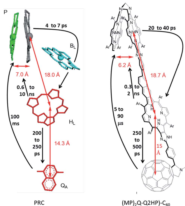
Fig. 1 (Left) Arrangement of the chromophores in the PRC from Rhodospseudomonas viridis , with the inter-chromophoric distances and process rates shown. (Right) The structure of (MP)_2Q-Q2HP-C_{60} (synthesised in this work) and the inter-chromophoric distances and analogous rates shown. P = 'special pair', B_L = auxiliary bacteriochlorophyll, H_L = primary-acceptor bacteriopheophytin, and Q_A = secondary-acceptor menaquinone; M = Zn(II) or 2H, Ar = 3,5-di- tert -butylphenyl.
