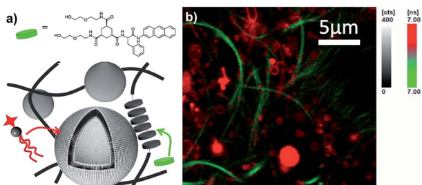
Fig. 7 (a) Preferential incorporation of fluorescent phospholipids (NBD-PE) in liposomes and 3a in the self-assembled fibers, (b) as evidenced by fluorescent lifetime imaging microscopy based on lifetime discrepancies ( \lambda_{\text{ex}} = 385 \text{ nm} , \lambda_{\text{em}} > 405 \text{ nm} , green reflects fluorescence lifetimes below 7 ns, red above 7 ns).
