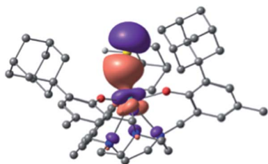
Fig. 6 Bonding \sigma orbital of [[(\text{Ad,MeArO})_3\text{tacn}]\text{U}(\text{SH})] (2).
