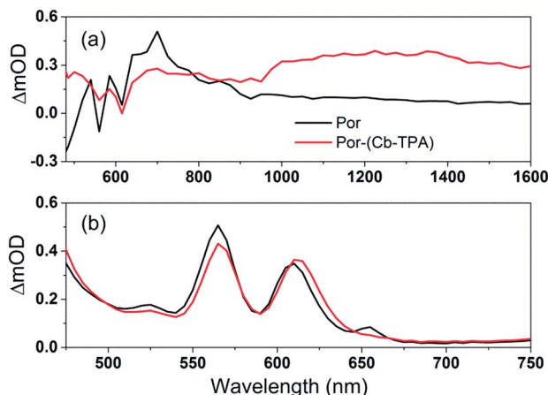
Fig. 5 (a) Transient absorption spectra of TiO 2 -Por and TiO 2 -Por-(Cb-TPA) in the presence of the inert electrolyte I 0 at 10 μs time delay following laser excitation (532 nm, 24–26 μJ cm -2 per pulse) and (b) absorbance of TiO 2 -Por and TiO 2 -Por-(Cb-TPA).
