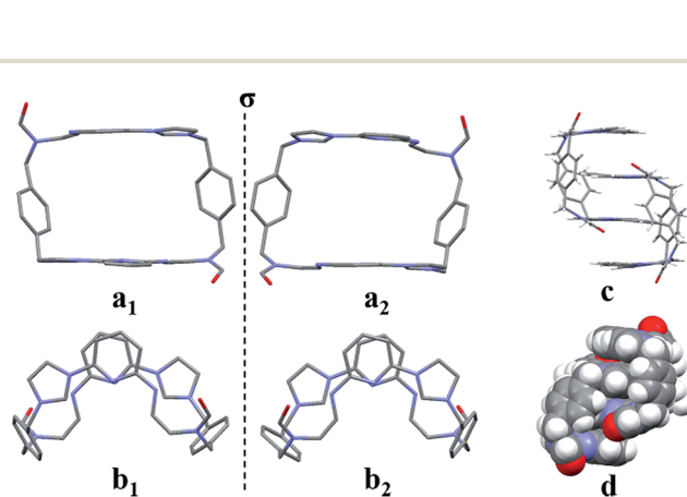
Fig. 2 Top ( a_1 and a_2 ) and side ( b_1 and b_2 ) views of the single crystal X-ray structure of [2^{2+} \cdot 2PF_6^- \cdot CH_3CN \cdot H_2O] showing the enantiomeric pair present in the crystal. Stick (c) and space-filling (d) views of these clip-like enantiomeric pairs. Counter ions and solvent molecules have been omitted for clarity.
