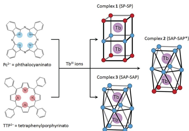
Scheme 1 Schematic illustration of dinuclear Tb III triple-decker complexes 1 – 3 , which show the three octa-coordination environments: SP–SP, SAP–SAP* and SAP–SAP, respectively, where SAP = square-antiprismatic and SP = square-prismatic.
