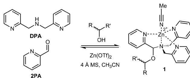
Fig. 1 Multicomponent hemiaminal ether assembly ( 1 ), formation from 2-pyridinecarbaldehyde ( 2PA ), di(picolyl)amine ( DPA ), \text{Zn}^{2+} , molecular sieves (3 Å), and a chiral alcohol analyte.
