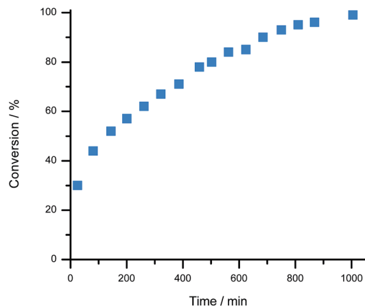
Fig. 3 Progress of H 2 activation by 1[BArCl] in the presence of the mediator, BArF 18 . H 2 (4 bar) was admitted to a sample of 1[BArCl] (0.028 mmol, 1.0 equivalents), BArF 18 (0.064 mmol, 2.3 equivalents), and 2,6-lutidine (0.048 mmol, 1.7 equivalents) in CD 2 Cl 2 and the formation of 1-H product was monitored using 1 H NMR spectroscopy.
