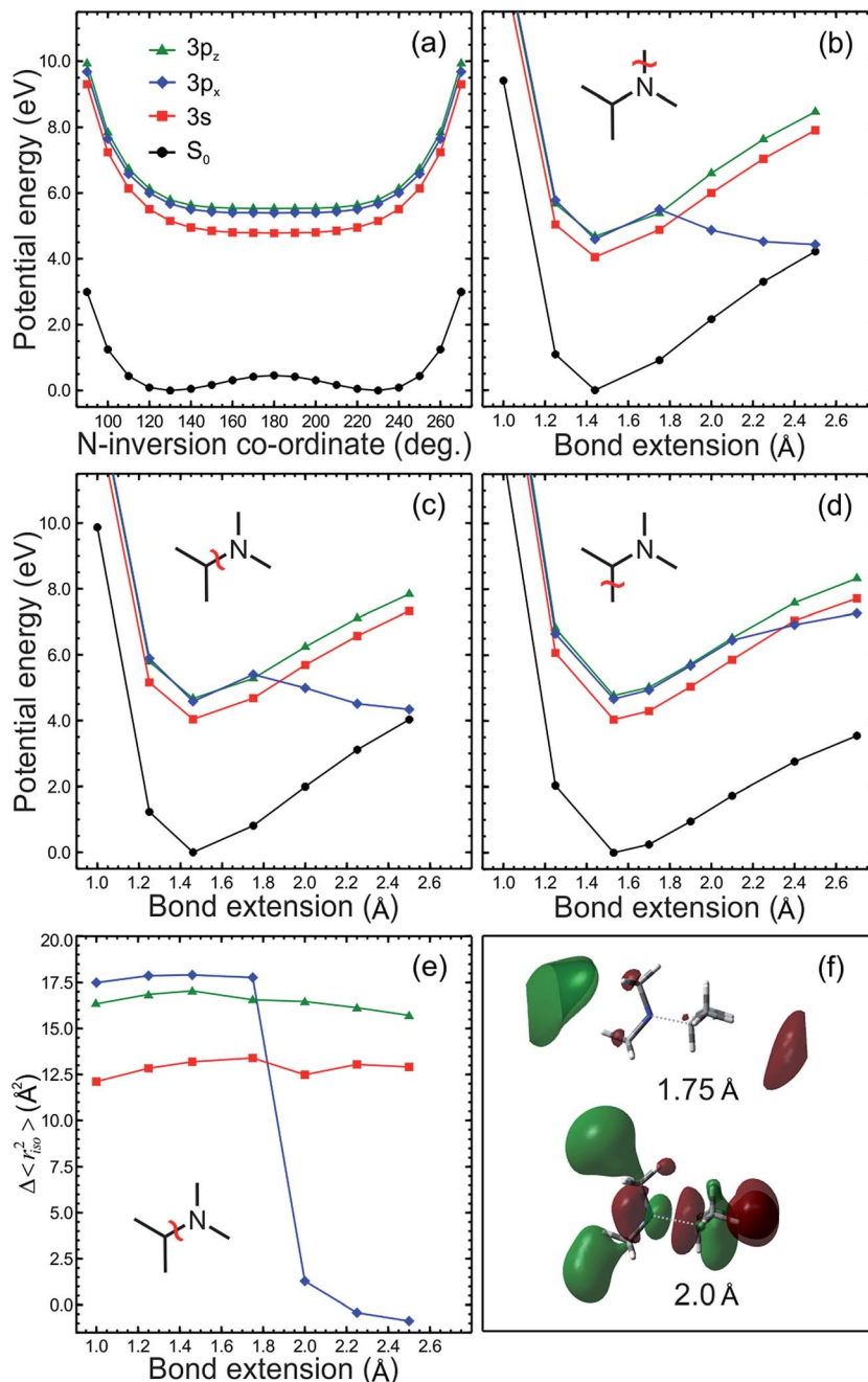
Fig. 9 EOM-CCSD/aug-cc-pVDZ potential energy cuts for DMIPA along (a) the nitrogen inversion (or “planarization”) coordinate, (b) the N -methyl bond, (c) the N -isopropyl bond, and (d) the C-methyl bond (corresponding to \alpha -cleavage). The relaxed excited state structure “Con 1” (see Fig. 8) was used as the starting reference geometry. Panel (e) shows the isotropic invariant of the excited-state second-moment of the electronic charge distribution with respect to the ground state along the N -isopropyl bond and (f) depicts the largest orbital transition in the EOM-CCSD eigenvectors at 1.75 and 2.0 Å, once again along the N -isopropyl bond.
