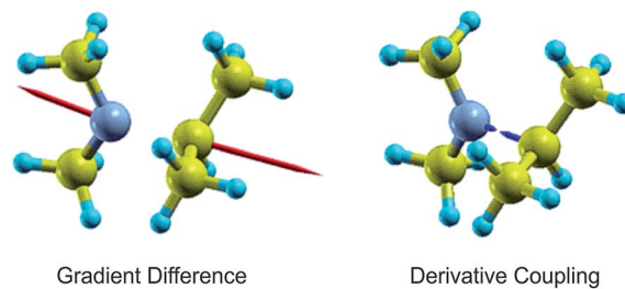
Fig. 10 Branching space vectors for the 3s/3p conical intersection (CI) as obtained from CASSCF calculations performed on DMIPA (described in the main text). The derivative coupling and gradient difference vectors define the directions in which the degeneracy is lifted when moving away from the CI point.
