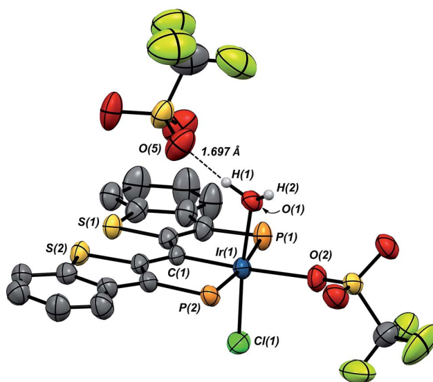
Fig. 7 Molecular structure of 8 . Hydrogen atoms, except for those on O(1), and the iso-propyl groups on phosphorus have been omitted for clarity. Displacement ellipsoids are shown at the 50% probability level. Selected bond lengths (Å): Ir(1)–P(1), 2.3642(13); Ir(1)–P(2), 2.3648(12); Ir(1)–C(1), 1.960(4); Ir(1)–O(1), 2.098(3); Ir(1)–O(2), 2.196(3); Ir(1)–Cl(1), 2.3200(12). Selected bond angles (°): C(1)–Ir(1)–O(1), 93.25(15); C(1)–Ir(1)–O(2), 175.46(16); O(1)–Ir(1)–O(2), 84.85(13); P(1)–Ir(1)–P(2), 171.34(4).
