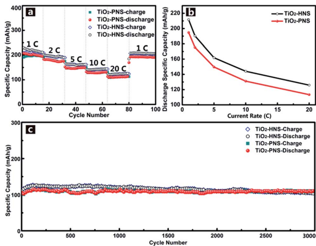
Fig. 6 (a) Cycling performance at various charge–discharge current rates of the \text{TiO}_2 -HNSs and \text{TiO}_2 -PNSs between 1.0 and 3.0 V. (b) Statistics of the discharge specific capacities at various current rates according to the rate performance in (a). (Each discharge capacity summarized here is the last cycle of each current rate.) (c) Long-term cycling performance of the \text{TiO}_2 -HNSs and \text{TiO}_2 -PNSs at a high current rate of 20 C for 3000 cycles.
