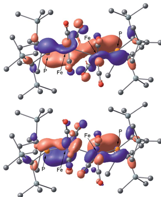
Fig. 4 Graphical representations of the DFT(PBE0)-derived HOMO (upper) and HOMO - 1 (lower) for 2_{\text{opt}} .
