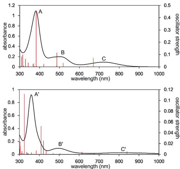
Fig. 3 UV-Vis-NIR spectra of the n -octane solution of 2 measured at 293 K (upper) and 353 K (lower). Solid red bars indicate the calculated transition of the 2_{\text{opt}} (upper) and 3_{\text{opt}} (lower).
