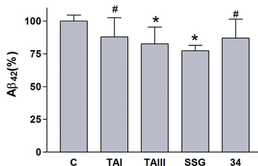
Fig. 9 In vivo A\beta_{42} -lowering activities of SSG and timosaponins. 3–5 month old C57BL/6 mice were dosed with vehicle (C), TAI, TAI, SSG or \alpha -, \beta -OH SSG (34) at 100 mg kg -1 by oral gavage for three times in 2 days. The levels of A\beta_{42} in the mouse brain were determined by ELISA. The number ( n ) of animals for vehicle control, TAI, TAI and SSG = 10; for 34, n = 6. Data represent means \pm standard deviations. Statistical significance in differences between vehicle control and treatment groups was determined by Student's test, #, P < 0.1; *, P < 0.05.
