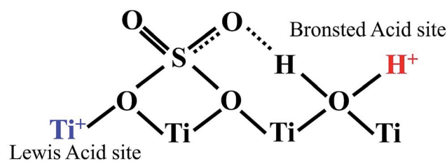
Fig. 7 Illustrative structure indicates the presence of both Bronsted and Lewis acid sites on the surface of TiO 2 –SO 4 .
