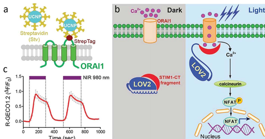
Fig. 3 (a) Schematic showing the interaction of streptavidin-conjugated UCNPs to engineered ORAI1 channels in the plasma membrane of HeLa cells. (b) Schematic of light-operated \text{Ca}^{2+} entry through engineered Opto-CRAC channels. (c) NIR light-induced reversible \text{Ca}^{2+} influx reported by red \text{Ca}^{2+} sensor, R-GECO1.2 in HeLa cells. 980 nm laser power density: 30 \text{ mW mm}^{-2} . Reprint with permission from ref. 32.
