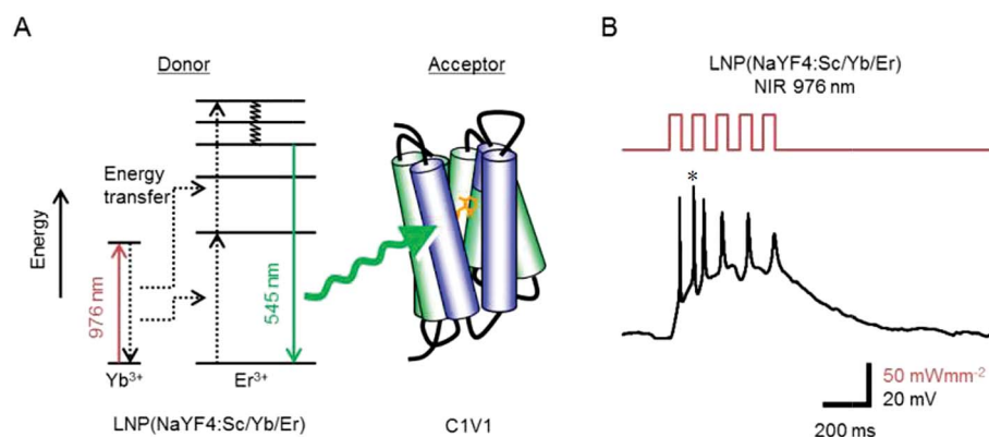
Fig. 4 \text{NaYF}_4:\text{Sc,Yb,Er} for NIR optogenetics. (A) The visible light emitted from donor \text{NaYF}_4:\text{Sc,Yb,Er} through upconversion of NIR light is absorbed by the acceptor (C1V1) to open the channel. (B) NIR flash-dependent firing of a cortical neuron through NIR optogenetics system. * denotes the asynchronous action potential. Reprint with permission from ref. 90.
