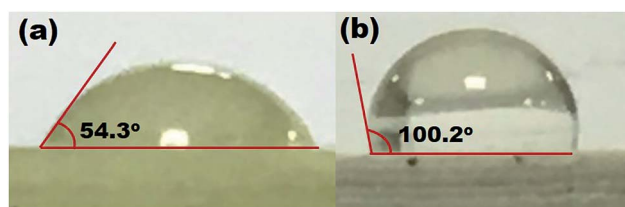
Fig. 5 Contact angle of water on the surface of (a) AP (b) APD-30 composite.
