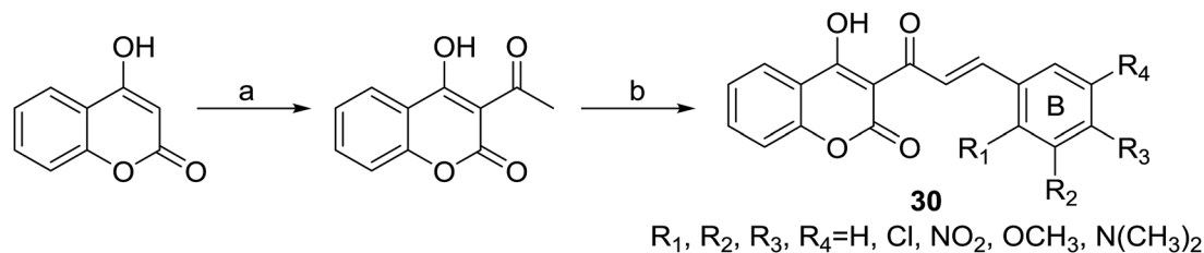
Scheme 1 Preparation for 3-cinnamoyl-4-hydroxy-2H-chromen-2-ones (30). (a) \text{POCl}_3 , reflux; (b) \text{CHCl}_3 , piperidine (catalytic), reflux.
