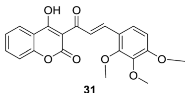
Fig. 4 Hybrid with 2,3,4-tri \text{OCH}_3 groups on B-ring of chalcone moiety.
