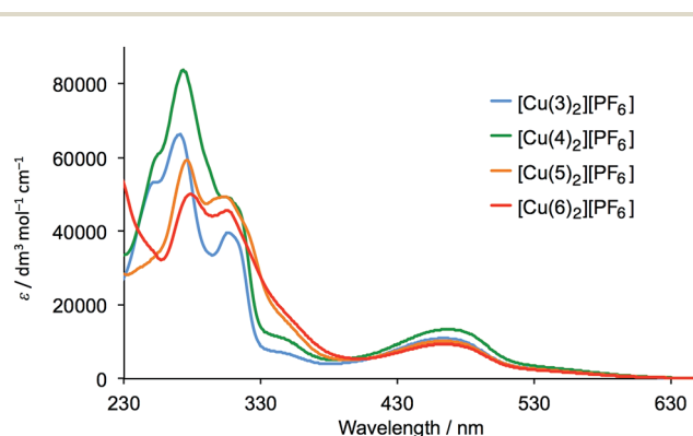
Fig. 2 Solution ( CH_2Cl_2 ) absorption spectra of complexes [Cu(L_{ancillary})_2][PF_6] with L_{ancillary} = 3-6 ( 5 \times 10^{-5} \text{ mol dm}^{-3} ).
