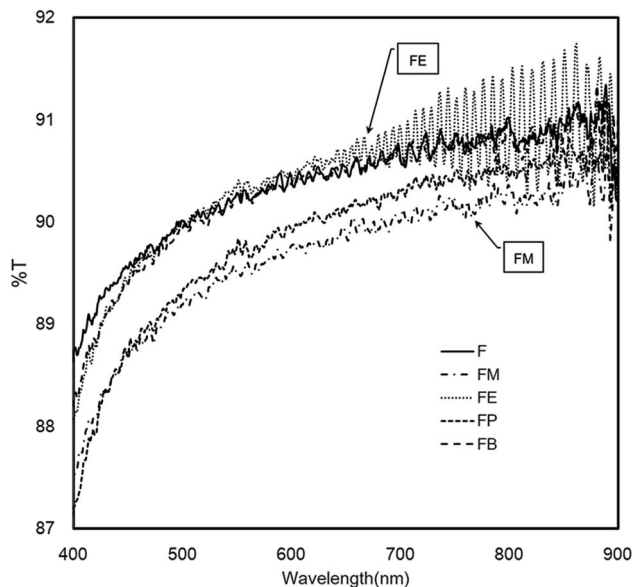
Fig. 7 UV/Vis spectra of silk fibroin films showing outstanding UV shield and optical transparency.
