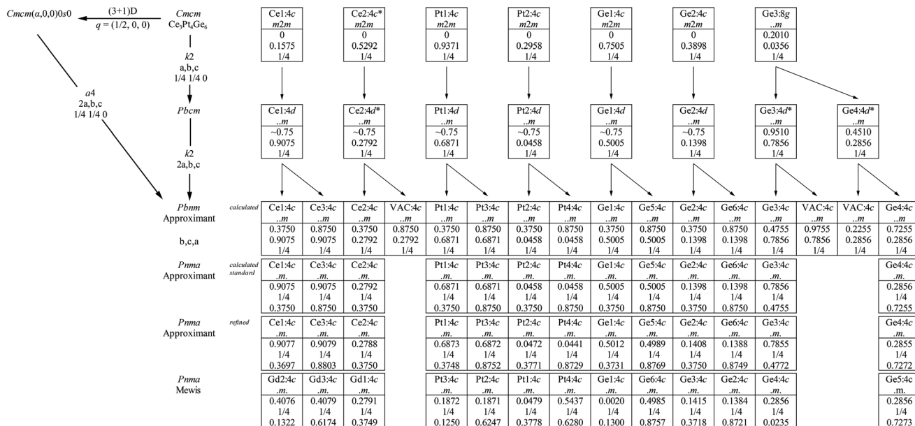
Fig. 5 Relation of the (3 + 1)D and 3D space groups of the modulated structure of Ce_3Pt_4Ge_6 . Group-supgroup scheme in the Bärnighausen formalism 40–43 for the subcell of Ce_3Pt_4Ge_6 (*occupancy parameter listed as 50% in the literature 24 ) and the supercell. The indices for the klassen-gleiche ( k ) symmetry reduction as well as the evolution of the atomic parameters are given. The index a is introduced for the formation of the approximant of the modulated structure. 39 The last line gives the atomic coordinates for Gd_3Pt_4Ge_6 , published by Mewis in space group Pnma . 25
