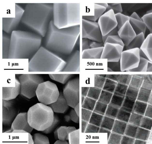
Fig. 1 Scanning electron microscopy (SEM) images of (a) TiO 2 polyhedrons (modified with permission from ref. 44, copyright 2008 Nature Publishing Group), (b) α-Fe 2 O 3 dodecahedra (modified with permission from ref. 51, copyright 2010 Wiley-VCH), field-emission scanning electron microscopy (FESEM) image of (c) Cu 2 O polyhedrons (modified with permission from ref. 53, copyright the Royal Society of Chemistry 2009), transmission electron microscopy (TEM) image of (d) ceria nanocubes (modified with permission from ref. 58, copyright 2006 American Chemical Society).
