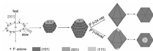
Scheme 2 Sketch of the growth mechanism of dodecahedral and octodecahedral α-Fe 2 O 3 particles (modified with permission from ref. 51, copyright 2010 Wiley-VCH).
