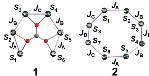
Fig. 6 Coupling schemes used for the magnetochemical modelling for compounds 1 and 2 .
