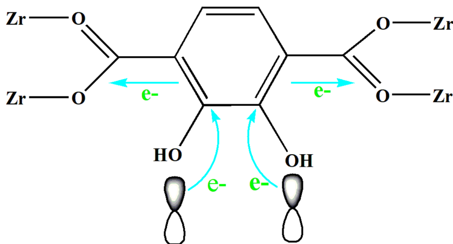
Fig. 10 Mechanism of hydroxy controlling photocatalytic activity.
