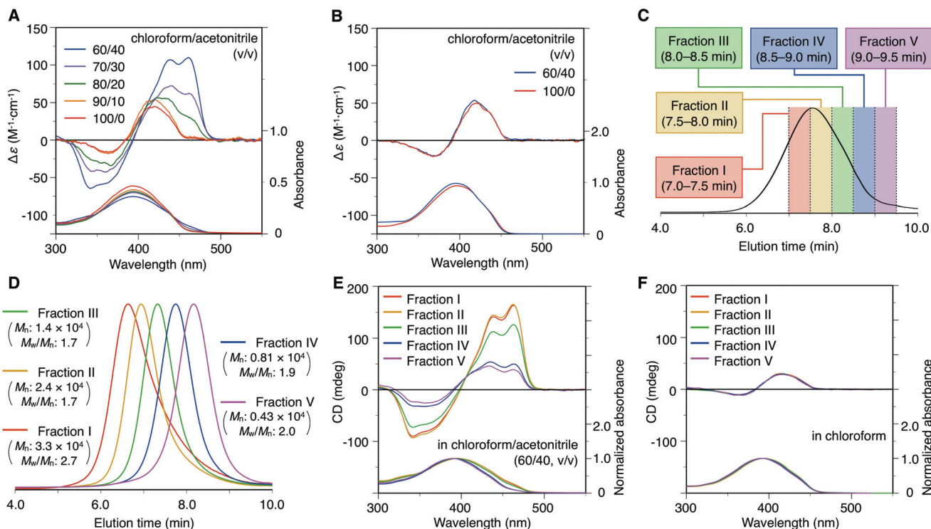
Fig. 2 (A, B) CD and absorption spectra of poly-9 (A) and mono-10 (B) in chloroform/acetoneitrile (100/0–60/40, v/v) at 25 °C. [Glucose unit] = 1.0 \times 10^{-4} \text{ M} . (C, D) SEC traces of the as-synthesized poly-9 ( M_n : 1.0 \times 10^4 \text{ g mol}^{-1} , M_w/M_n : 3.3) (C) and its fractionated components with different molecular weights (D) (eluent, chloroform; polystyrene standards). (E, F) Molecular weight dependency of the CD and absorption spectra of poly-9 in chloroform/acetoneitrile (60/40, v/v) (E) and chloroform (F) at 25 °C. To allow comparison of the CD intensities, the CD spectra were normalized with respect to the absorbance at the absorption maximum wavelength. The corresponding CD (unprocessed) and absorption (not normalized) spectra are shown in Fig. S6.†
