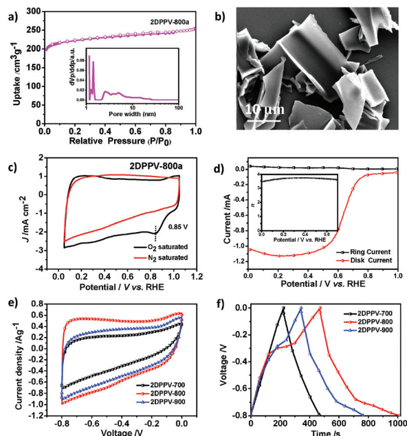
Fig. 3 (a) Nitrogen adsorption–desorption isotherms of 2DPPV-800a (inset: pore size distribution); (b) SEM image of 2DPPV-800a; (c) CV curves of 2DPPV-800a in \text{N}_2 -saturated and \text{O}_2 -saturated 0.1 M KOH at a scan rate of 50 \text{ mV s}^{-1} ; (d) RRDE voltammogram for 2DPPV-800a in 0.1 M KOH solution saturated with \text{O}_2 (the electrode rotation rate was 1600 rpm and the Pt ring electrode was held at 0.5 V, inset: electron transfer number of 2DPPV-800a as a function of potential); (e) CV curves of 2DPPV-X ( X = 700, 800, 900 ) at 5 \text{ mV s}^{-1} in 6 M KOH aqueous solution; and (f) galvanostatic charge/discharge curves for 2DPPV-X ( X = 700, 800, 900 ) at a current density of 0.5 \text{ A g}^{-1} .
