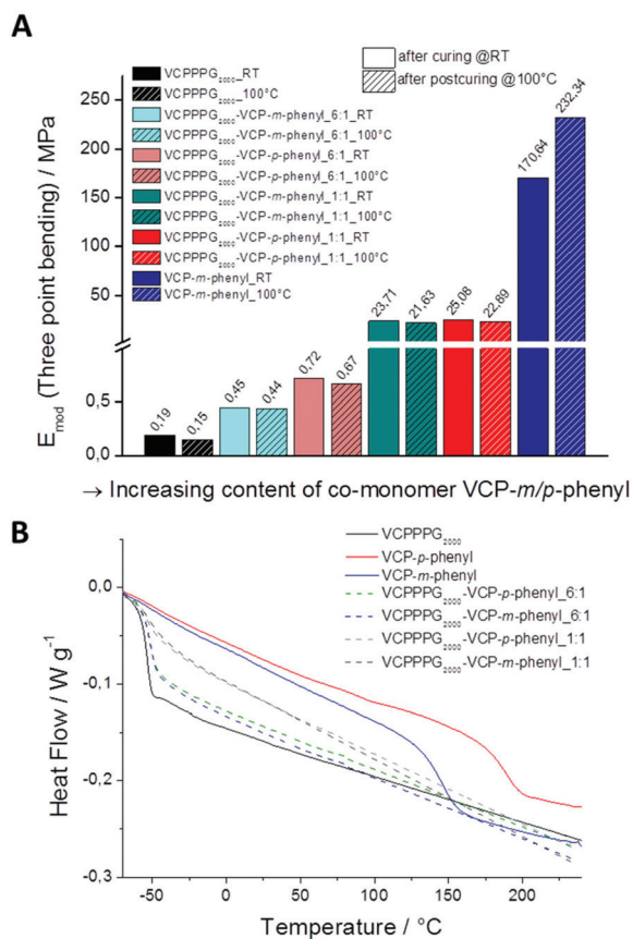
Fig. 4 (A) Determined E-moduli of cured VCP-phenyl specimens, as well as by co-networks in ratios of 6 : 1 and 1 : 1 of VCP-phenyl, VCP- m -phenyl and VCP- p -phenyl. With increasing content of the co-monomer VCP- m/p -phenyl, the moduli could be raised up to 1200 times to higher values. (B) Second DSC heating trace of cured VCP specimens, illustrating the glass transition T_g of the cured samples.
