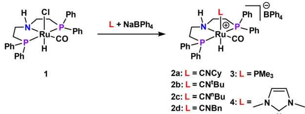
Scheme 1 Synthesis of 2a, 2b, 2c, 2d, 3 and 4.
