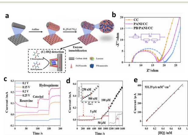
Fig. 8 (a) Synthesis process of the HQ biosensor using PB/PANI, (b) EIS diagram, which involves the three mentioned electrodes, spanning a frequency range from 0.1 \text{ Hz} to 1 \text{ MHz} , (c) amperometric responses at different operating potentials, (d) the signals' reactions, and (e) linear calibration of the Lac-PB/PANI/CC biosensor at 0.15 \text{ V} in PBS, with insets displaying the detection duration and a magnification of the curve from 100 to 600 s. Reprinted from ref. 132, copyright (2023), with permission from Elsevier.
