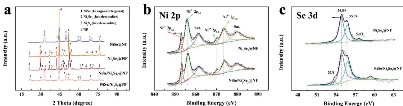
Fig. 2 Spectroscopic characterizations. XRD patterns (a) of Ni3Se2@NF, NiSe@NF, NiSe/Ni3Se2@NF, and NiSe/Ni3S2@NF. (b) Ni 2p spectra. (c) XPS fitting of Se 3d peaks of NiSe/Ni3Se2@NF and Ni3Se2@NF.
