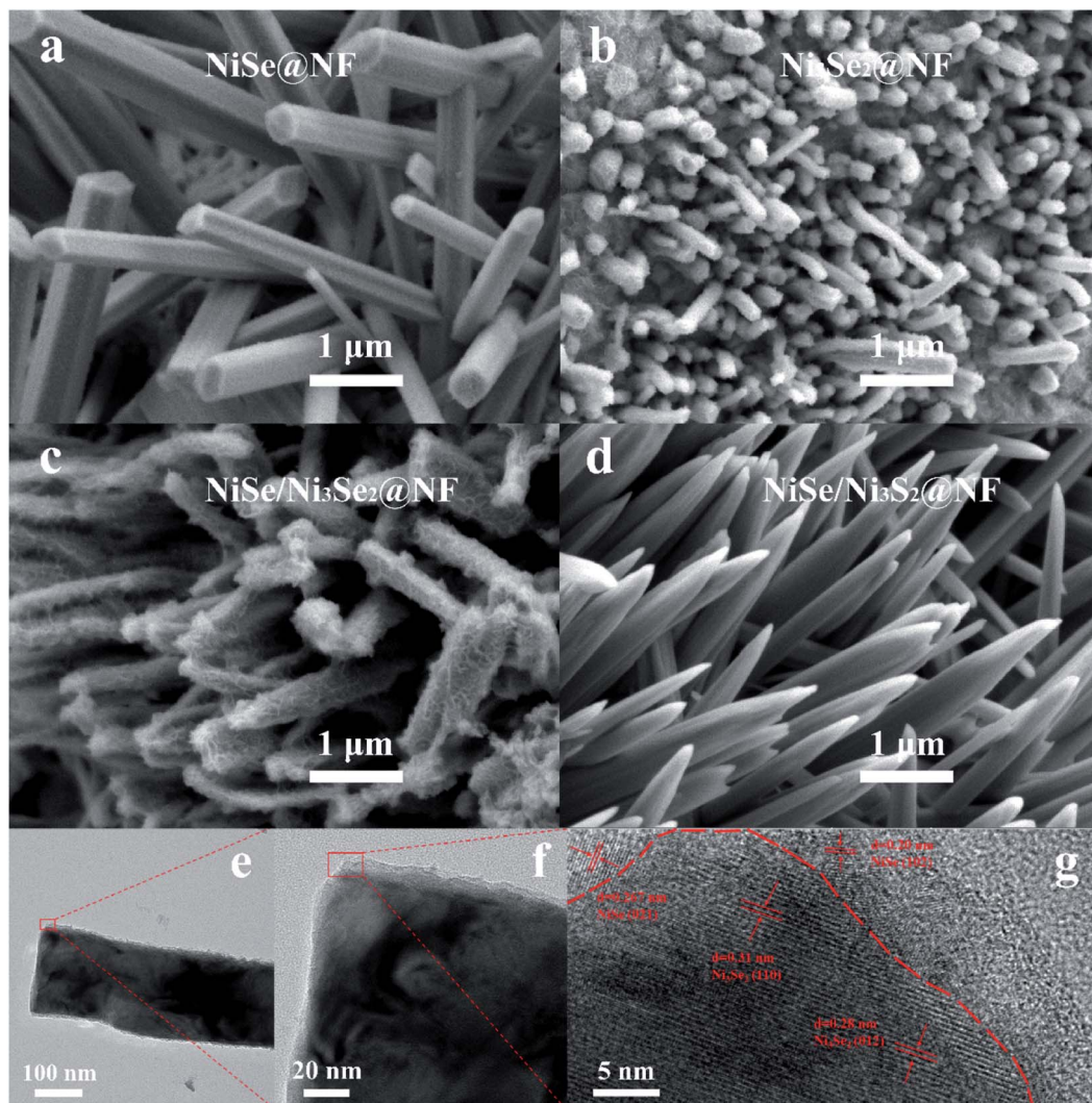
Fig. 1 Morphological and structural characterizations. SEM images of NiSe@NF (a) Ni3Se2@NF (b) NiSe/Ni3Se2@NF (c) NiSe/Ni3S2@NF (d) and high-resolution TEM images of NiSe/Ni3Se2@NF (e–g).
