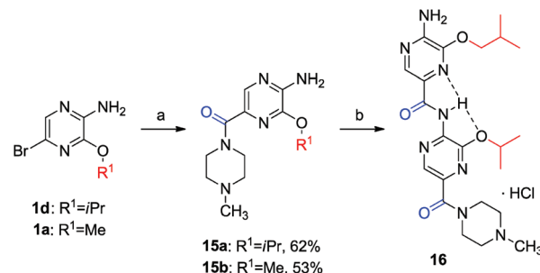
Scheme 6 Synthesis of dimer HCl salt by piperazine end-cap. Reagents and conditions: (a) N -methylpiperazine, Pd(OAc) 2 , xantphos, CO, Na 2 CO 3 , toluene, 100 °C. (b) 1. 2b , Pd(OAc) 2 , xantphos, CO, Na 2 CO 3 , toluene, 100 °C, 17% (43% with recovery of 15a ). 2. TFA, DCM, 97%. 3. HCl, dioxane, quant.
