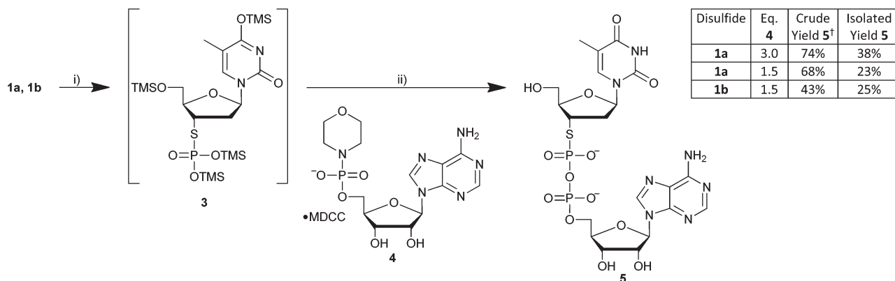
Scheme 1 Synthesis of dTSppA. Reagents and conditions: (i) (\text{TMSO})_3\text{P} , BTMSA, \text{CHCl}_3 , RT, 30 min; (ii) (a) 4 , tetrazole, \text{MgCl}_2 \cdot 6\text{H}_2\text{O} , \text{H}_2\text{O} , LAG, 30 Hz, 90 min, (b) \text{H}_2\text{O} , \text{CH}_3\text{OH} , \text{CH}_3\text{CN} (from 1b ); or \text{H}_2\text{O} (from 1b ). Key: MDCC = 4-morpholine- N,N' -dicyclohexylcarboxamidinium; †calculated using integration of the \beta -phosphoryl resonance (based upon 100% efficient M–A reaction).
