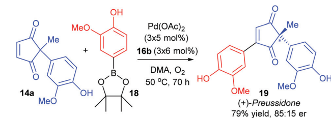
Scheme 11 Synthesis of (+)-preussidone using enantioselective oxidative Heck reaction.
