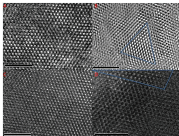
Fig. 5 The HR-TEM images of MoS_2 exfoliated with sodium naphthalenide (A) and butyllithium (B). The dominant occurrence of the 1T form is clearly seen in the MoS_2 -NAPH sample (panel A) while for the sample MoS_2 -BuLi (panel B) both phases, 2H and 1T (1T phase marked by blue triangle), coexist in comparable amounts. WS_2 exfoliated with sodium naphthalenide corresponds to panel C and with butyllithium to panel D where both 2H and 1T forms can be identified (1T phase marked by a blue triangle). The scale bar corresponds to 2 nm.
