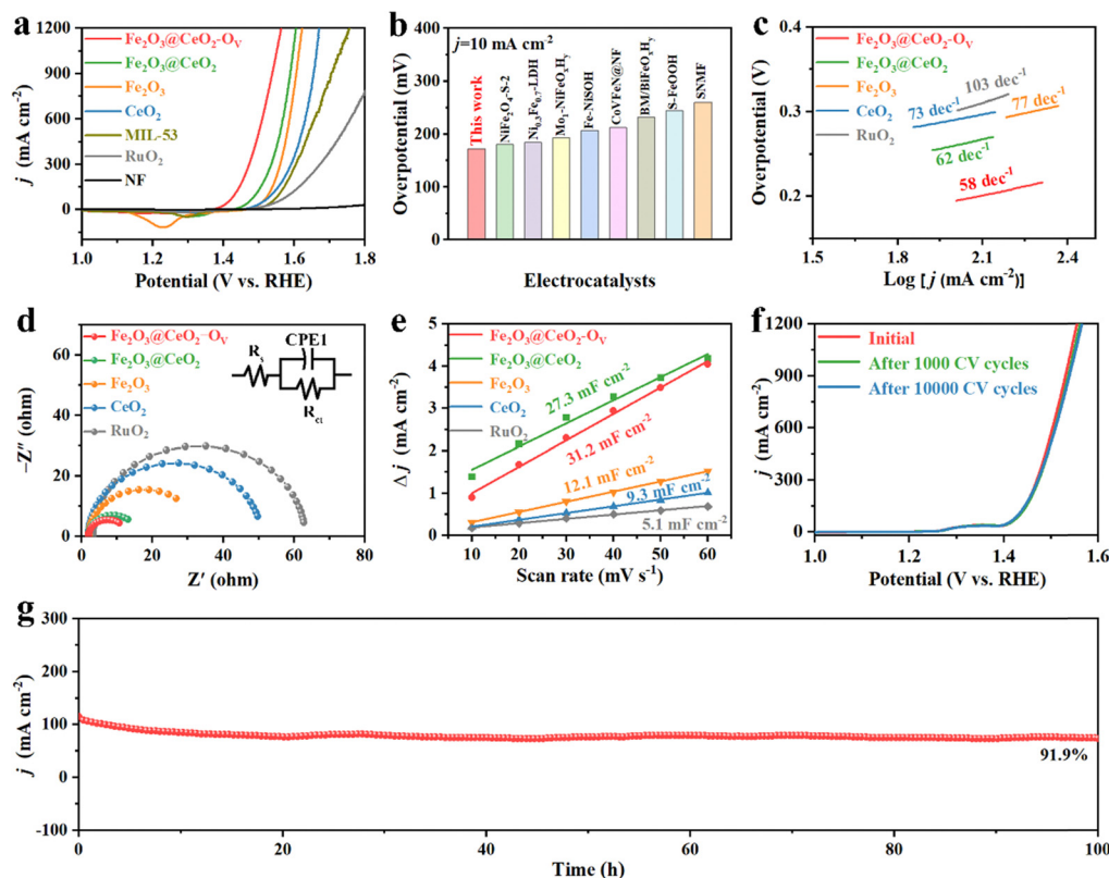
Fig. 3 OER performance of the prepared electrodes. (a) LSV negative scan curves in 1.0 M KOH with 90% iR compensation. (b) Comparison of overpotentials at a current density of 10 \text{ mA cm}^{-2} with reported Fe-based electrocatalysts. (c) Corresponding Tafel plots. (d) EIS plots of samples, and the insert shows the equivalent circuit. (e) C_{dl} calculations of the Fe 2 O 3 @CeO 2 -O v , Fe 2 O 3 @CeO 2 , Fe 2 O 3 , CeO 2 and RuO 2 samples. (f) LSV curves of Fe 2 O 3 @CeO 2 -O v , before and after 1000 and 10 000 CV cycles in 1.0 M KOH for the OER. (g) Chronoamperometric stability tests of Fe 2 O 3 @CeO 2 -O v .
