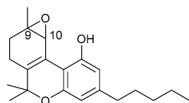
34 9,10-Anhydrocannabitriol [108]
