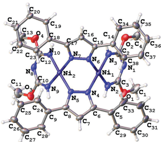
Fig. 4 Molecular structure of 3 with the atomic numbering scheme. Thermal ellipsoids are given at the 50% probability level.
