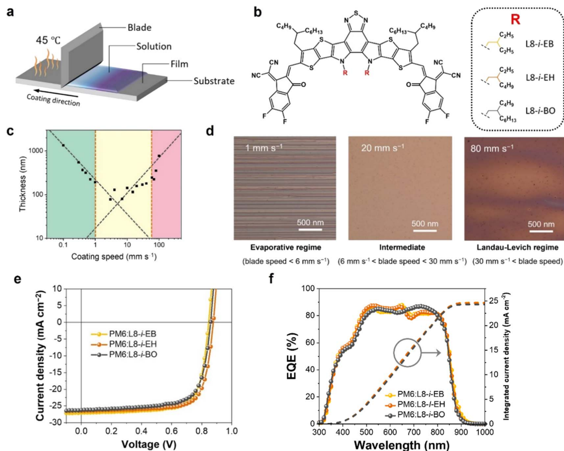
Fig. 1 (a) The schematic illustration of the blade-coating process. (b) Chemical structures of L8-i-EB, L8-i-EH, L8-i-BO, and PM6. (c) Thickness of active layers depending on blade speed. (d) Optical microscopy images of films fabricated at a speed within the evaporative regime, intermediate, and Landau–Levich regime. (e) J – V curves and (f) EQE spectra and integrated current density curves of the optimized PM6:NFA-based device.
