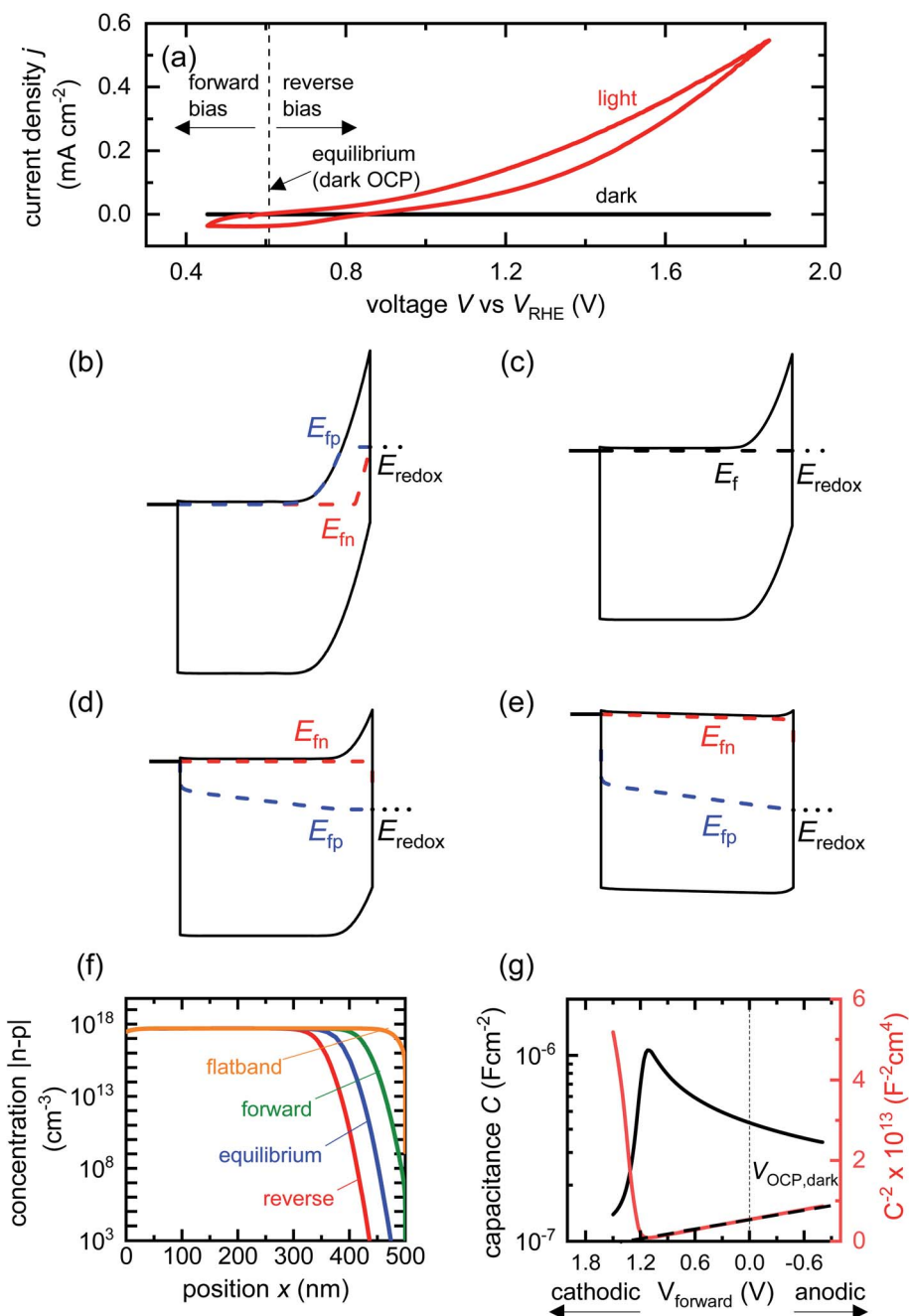
Fig. 2 (a) Cyclic voltammetry curves of a BiVO 4 photoanode in the dark and under one sun illumination. Also shown are the voltages corresponding to large forward bias, equilibrium (dark open-circuit potential) and deep reverse bias (anodic voltages). Simulated band diagrams of a doped BiVO 4 photoanode ( N_d = 5 \times 10^{17} \text{ cm}^{-3} ) in the dark at (b) reverse bias, (c) equilibrium, (d) forward bias and (e) flatband conditions. (f) Shows the net concentration [n-p] in the photoanode as a function of position for the different bias situations in (b)–(e). The net concentration is dominated by the electron density, which is several orders of magnitude larger than the hole density in all cases. (g) Capacitance step and corresponding Mott–Schottky plot (dashed line shows linear Mott–Schottky region) from a simulated small-perturbation capacitance–voltage measurement ( 10^3 \text{ Hz} ). This capacitance corresponds to the depletion capacitance. Simulation parameters are shown in Table S2 in the ESI.†
