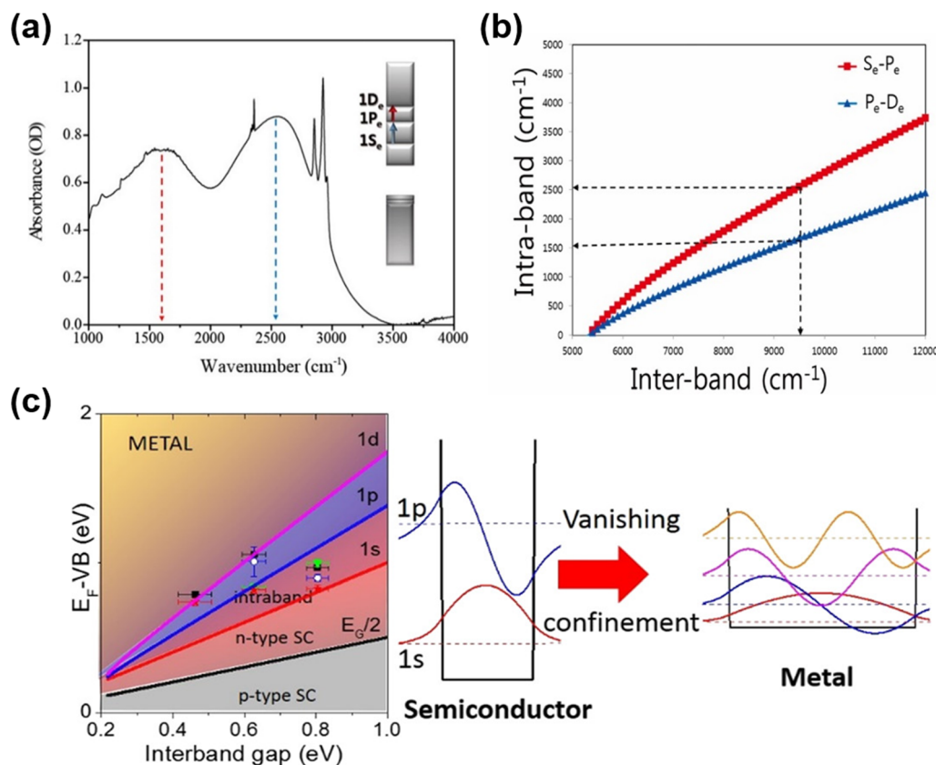
Fig. 5 Intra-band transitions of HgS and HgSe QDs. (a) Intra-band transitions (1S e -1P e and 1P e -1D e ) for n-doped HgS QDs. (b) Comparison of the inter-band and the first intra-band transition energies for a given size calculated for HgS. (a and b) Are reproduced from ref. 72 with permission from American Chemical Society, copyright 2016. (c) Successive filling of the lower electron excited states results in increasing n-doped characteristics. p-Type behaviour gives way to ambipolar, then n-type (introducing the possibility of intra-band transitions as the 1S e level is filled), and eventually plasmonic behaviour at higher occupancies. As the QD size increases and the inter-bandgap energy decreases, these transitions in behaviour occur at lower energies. The data points correspond to QDs of various sizes and ligand doping treatments. Reproduced from ref. 78 with permission from American Chemical Society, copyright 2017.
