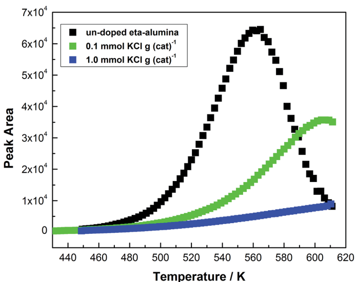
Fig. 6 Plot of dimethyl ether concentration as a function of reaction temperature for (a) the un-doped \eta -alumina catalyst (black squares), (b) \eta -alumina catalyst + 0.1 \text{ mmol KCl g(cat)}^{-1} (green squares), and (c) \eta -alumina catalyst + 1.0 \text{ mmol KCl g(cat)}^{-1} (blue squares).
