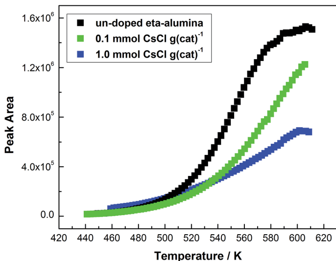
Fig. 5 Plot of methyl chloride concentration as a function of reaction temperature for (a) the un-doped \eta -alumina catalyst (black squares), (b) \eta -alumina catalyst + 0.1 \text{ mmol CsCl g(cat)}^{-1} (green squares), and (c) \eta -alumina catalyst + 1.0 \text{ mmol CsCl g(cat)}^{-1} (blue squares).
