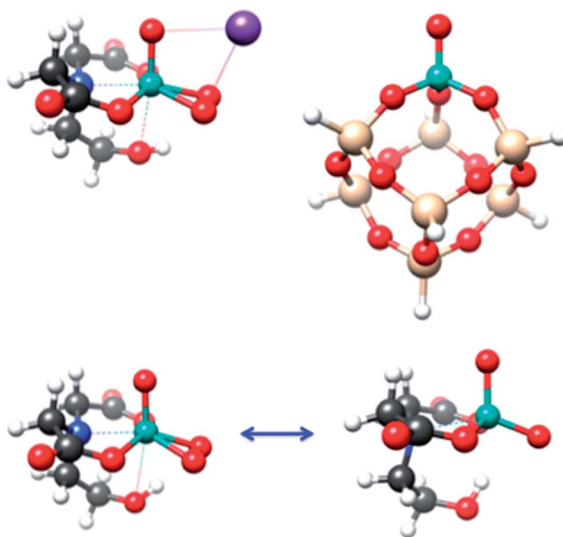
Fig. 1 Top left: The molecular structure of K[VO(O_2)Hseida] . Top right: Representative model structure of monomeric silica supported vanadia catalyst, VS_{17}H_7O_{13} . Bottom: Two possible active forms of the molecular catalyst; [VO(O_2)Hseida]^- (left) and oxygen deficient [VO(O)Hseida]^- (right). Atom colouring: H (white), C (gray), O (red), N (blue), V (cyan), Si (light yellow) and K (purple).
